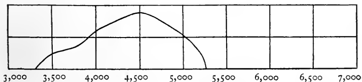
FIG. II. DIFFERENT TYPES OF PLATE SENSITIVENESS CURVES TO DAYLIGHT
